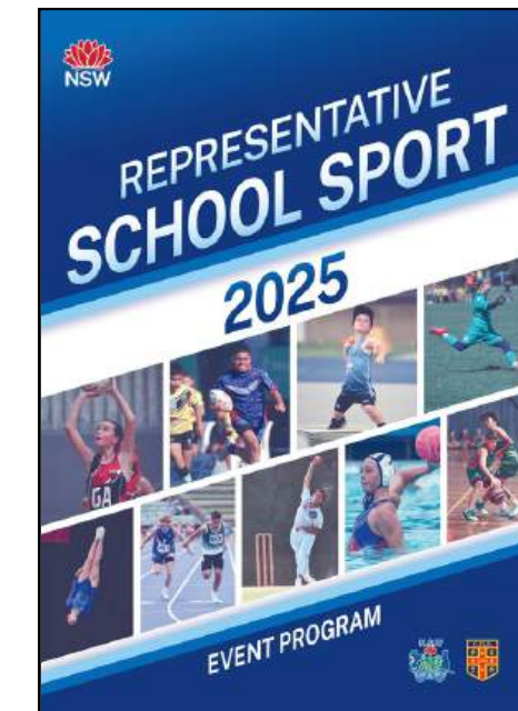
Program example
